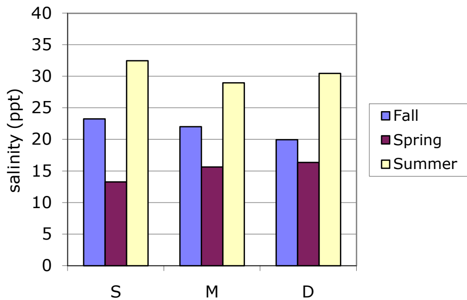
Littleneck Rd., Ipswich 1999-2008 Seasonal Average Salinity vs. Well Depth
