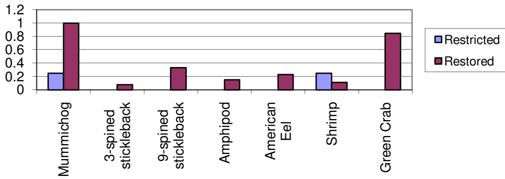
Eastern Point Gloucester Percent Frequency Downstream Pre and Post Restoration (2002-2008)
