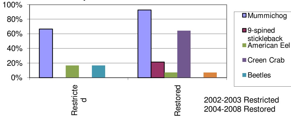
Eastern Point Gloucester Percent Frequency of Different Upstream Area Restricted vs. Restored
