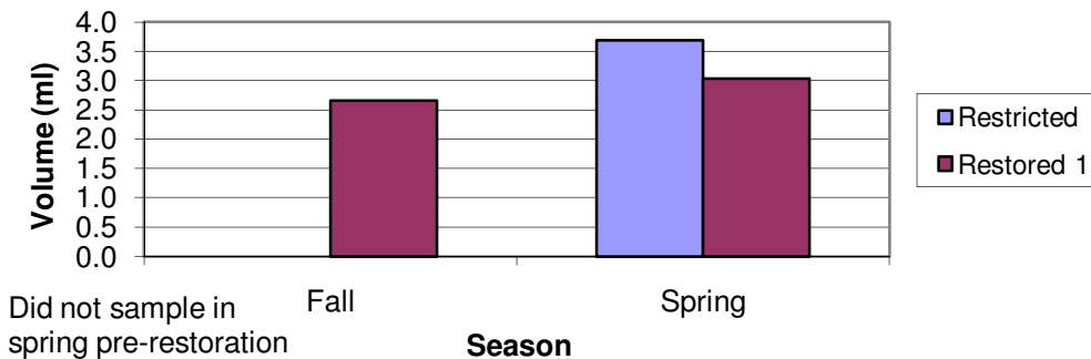
Eastern Point, Gloucester, MA Average Volume Mummichogs vs. Season 2002-2008
