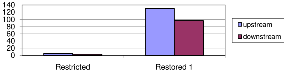
Eastern Point, Gloucester Average Volume of Mummichogs vs. treatment vs. location 2002-2003=restricted, 2004-2008= restored
